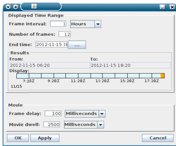
Figure 4.2.6-1 :Configure animation
