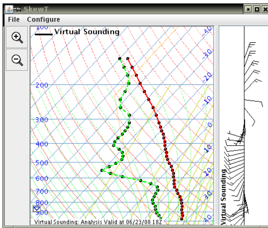
Figure 4.12-1: Virtual Sounding/Skew T
