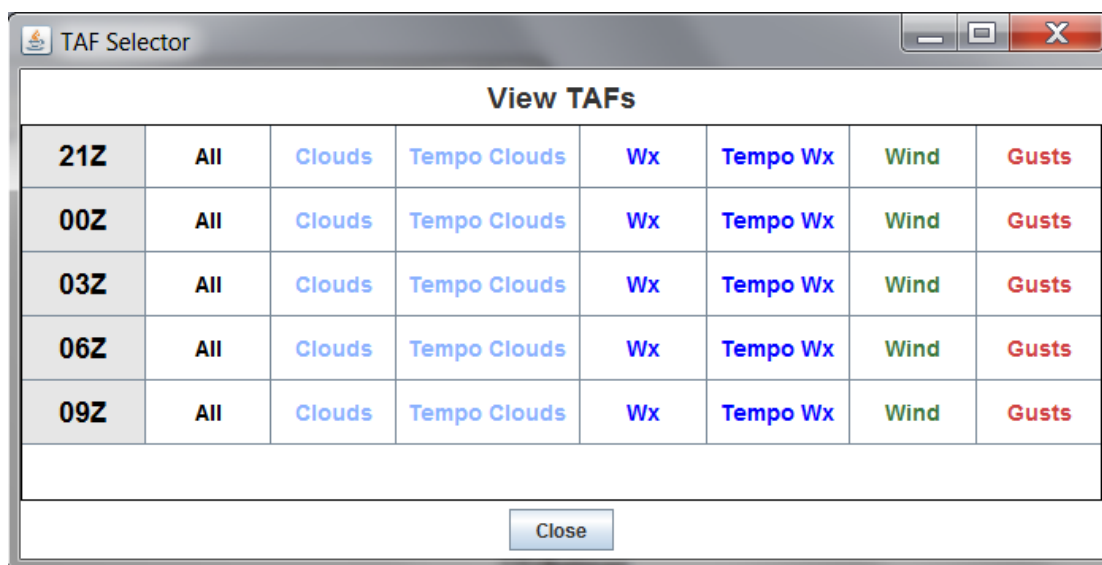
Figure 4.2.6-5 :TAF Selector
